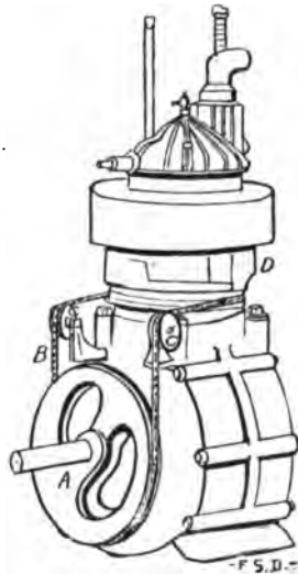
FIG. 298.—The "Kainz" Motor, showing rotary cooling fan about the cylinder. The fan cylinder, D, is rotated by a cord, B, turned by the pulley, A, on the crank shaft and passing over pulleys, C, C.
